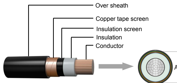
Cable construction
